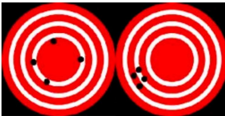
Figure 1.14: A visual analogy of accuracy and precision. Left target: High accuracy but low precision; Right target: low accuracy but high precision. The results of calculations or a measurement can be accurate but not precise; precise but not accurate; neither accurate nor precise; or accurate and precise. A collection of bulls eyes right around the center of the target would be both accurate and precise.
