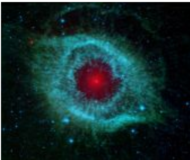
Figure 1.12: The Helix nebula, located about 700 light-years away in the constellation Aquarius, belongs to a class of objects called . Planetary nebulae are the remains of stars that once looked a lot like our sun. When sun-like stars die, they puff out their outer gaseous layers. These layers are heated by the hot core of the dead star, called a white dwarf, and shine with infrared and visible colors. Scientists can study the birth and death of stars by analyzing the types of light that are emitted from nebulae.
