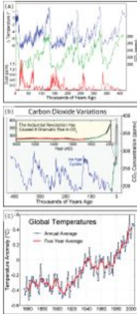
Figure 11.53: (A) Changes in CO levels (green) are clearly associated with temperature changes (blue); the graph shows the four major Ice ages of the Pleistocene. Graphs B (long time scale) and C (recent time) show increases in CO and global temperature over the past 150 years, suggesting that the Industrial Revolution, which began our major fossil fuel burning and release of CO, may account for much of the increase in temperature – a new, human-induced global warming.
